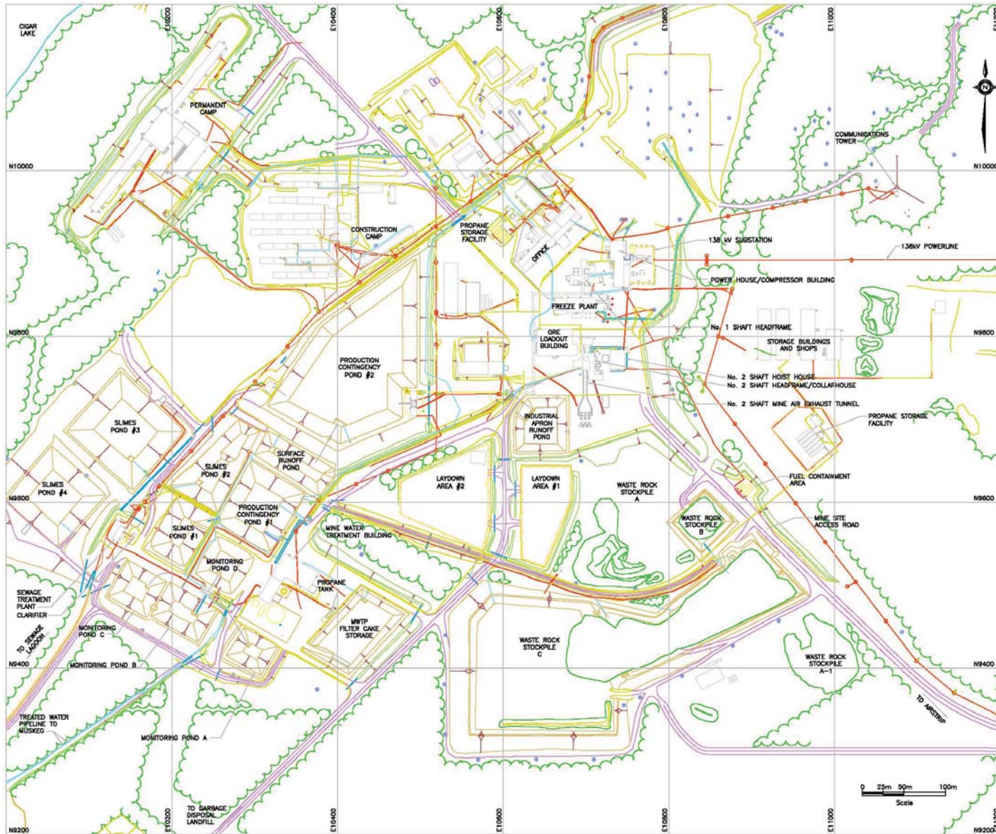
Figure 5-2: Site Plan Showing Existing and Planned Surface Facilities
