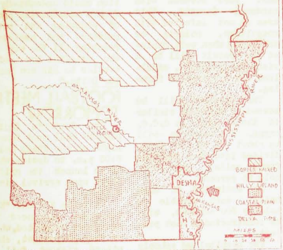
MAJOR AG-SOIL AREAS IN ARKANSAS
