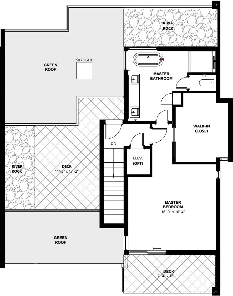
Upper Level
