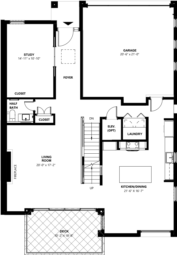
Main Level
