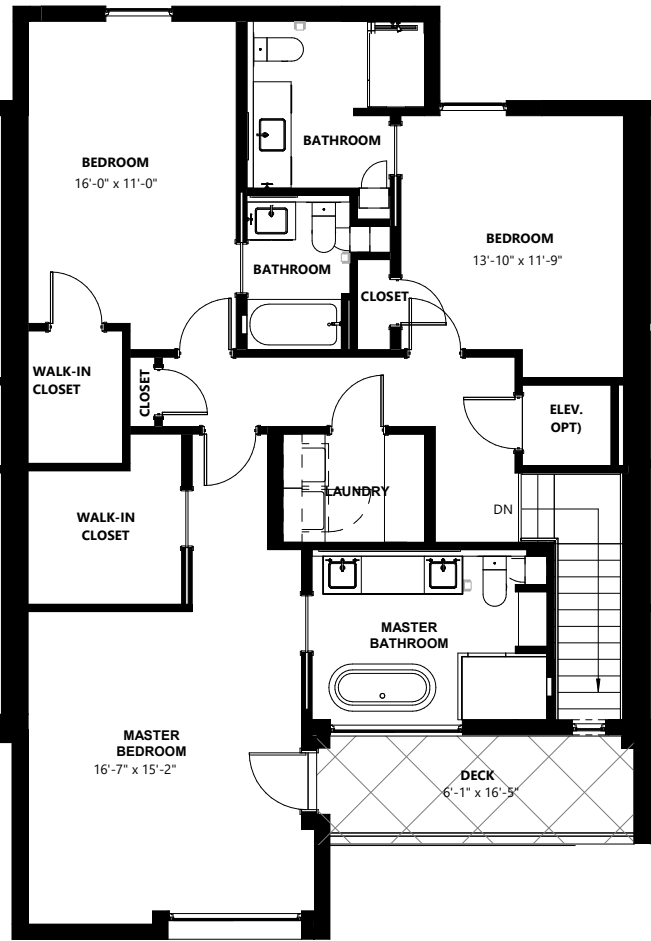
Upper Level
