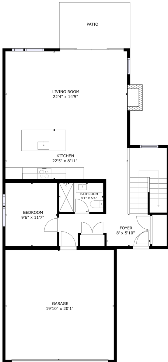
FLOOR 1
