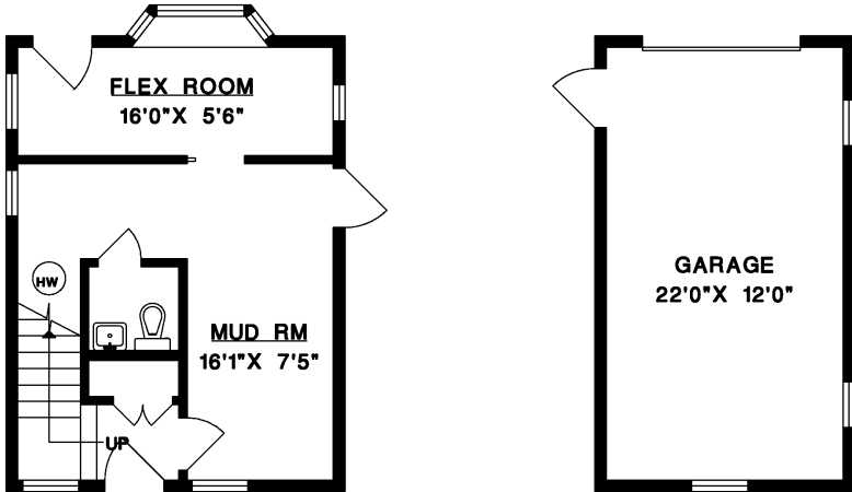
LOWER FLOOR
