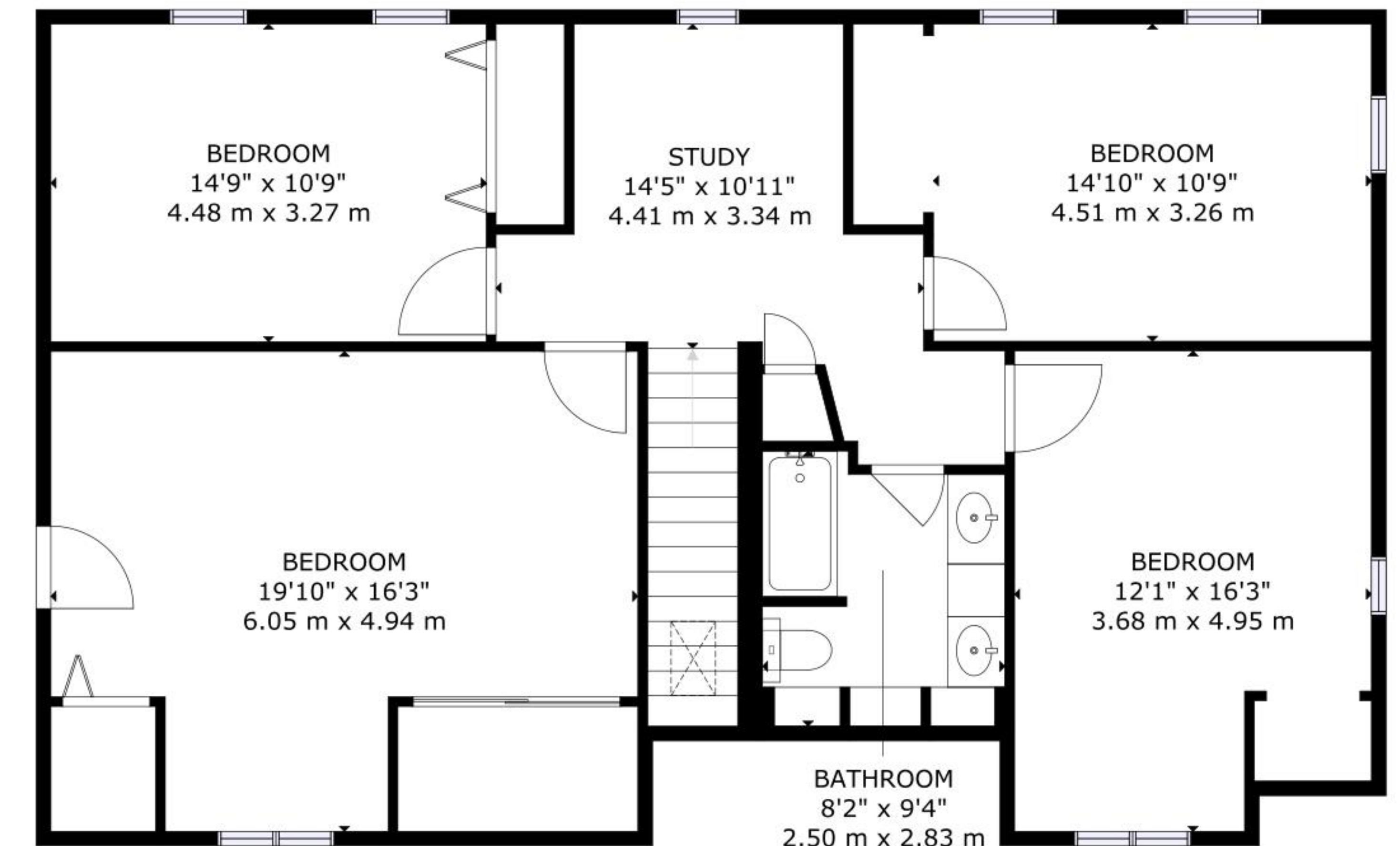
FLOOR 2
