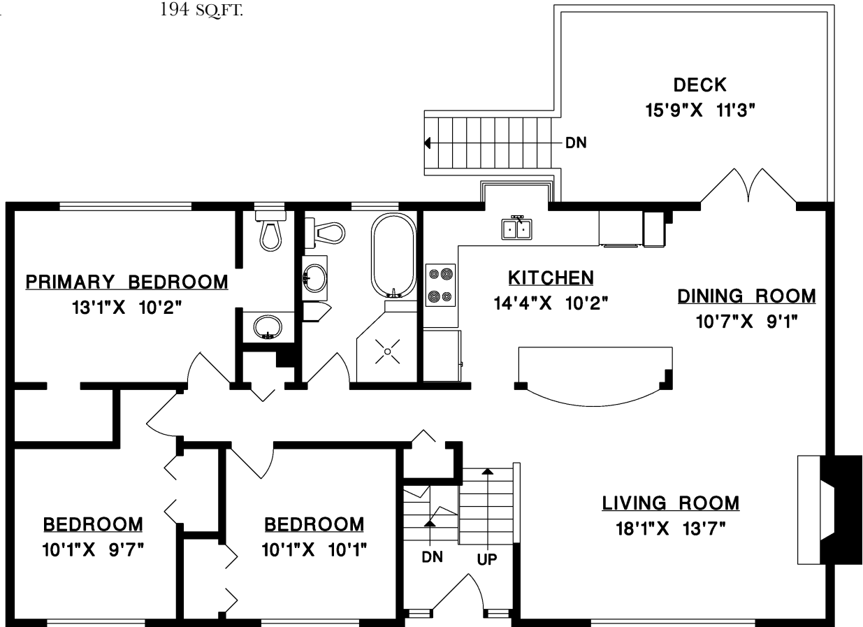
MAIN FLOOR
