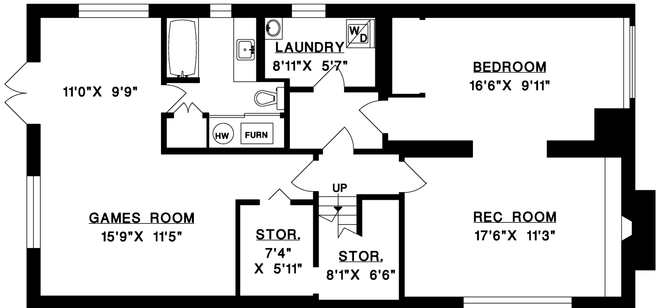
LOWER FLOOR
