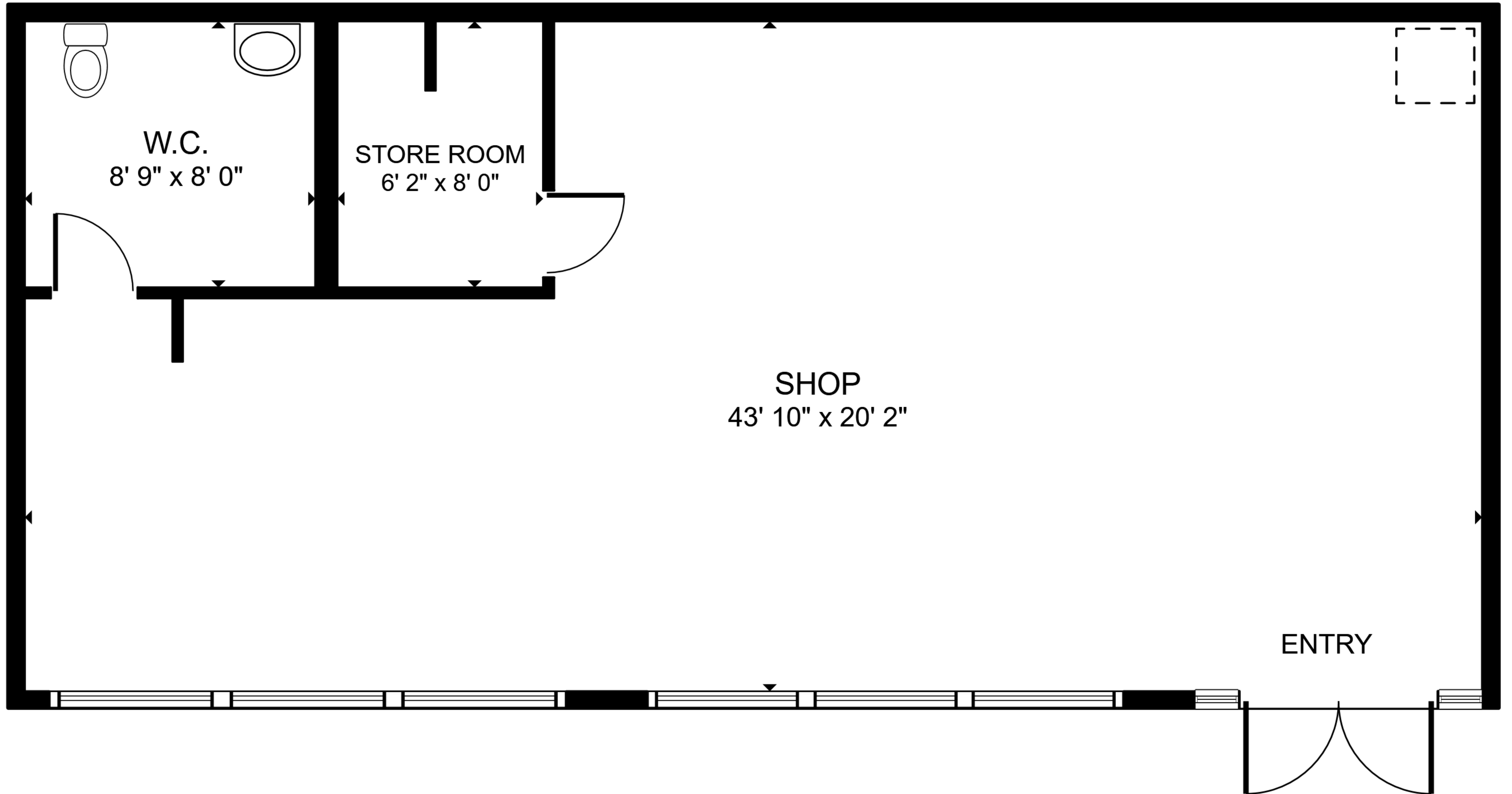
FLOOR PLAN
