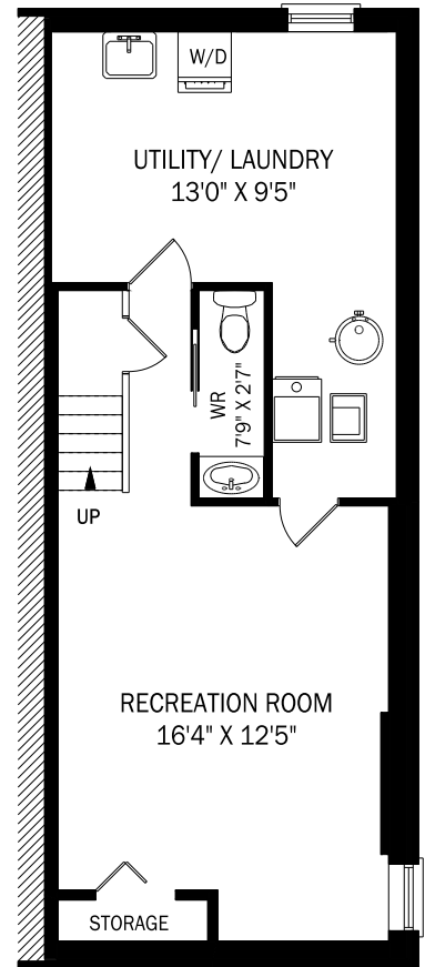
CEILING HEIGHT 6'1" LOWER LEVEL - 506 SQUARE FEET
