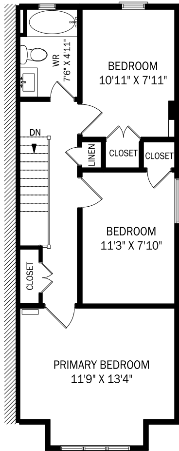
CEILING HEIGHT 8'5" SECOND FLOOR - 524 SQUARE FEET
