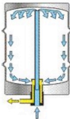
Blow Out of Acid with Sterile Air
