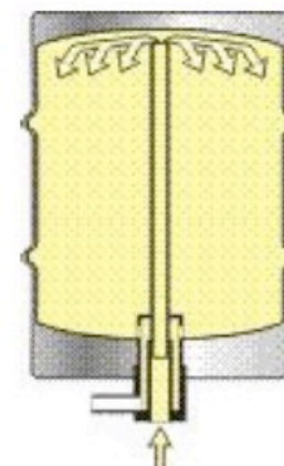
Counter- Pressurizing of CO 2 to Filling Pressure
