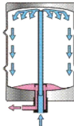
Blow Out Caustic with Sterile Air
