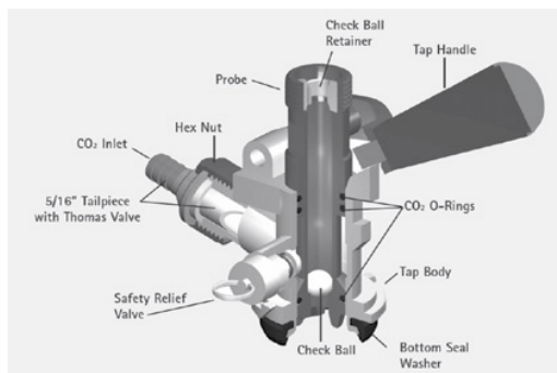
D-System Coupler Cross Section
