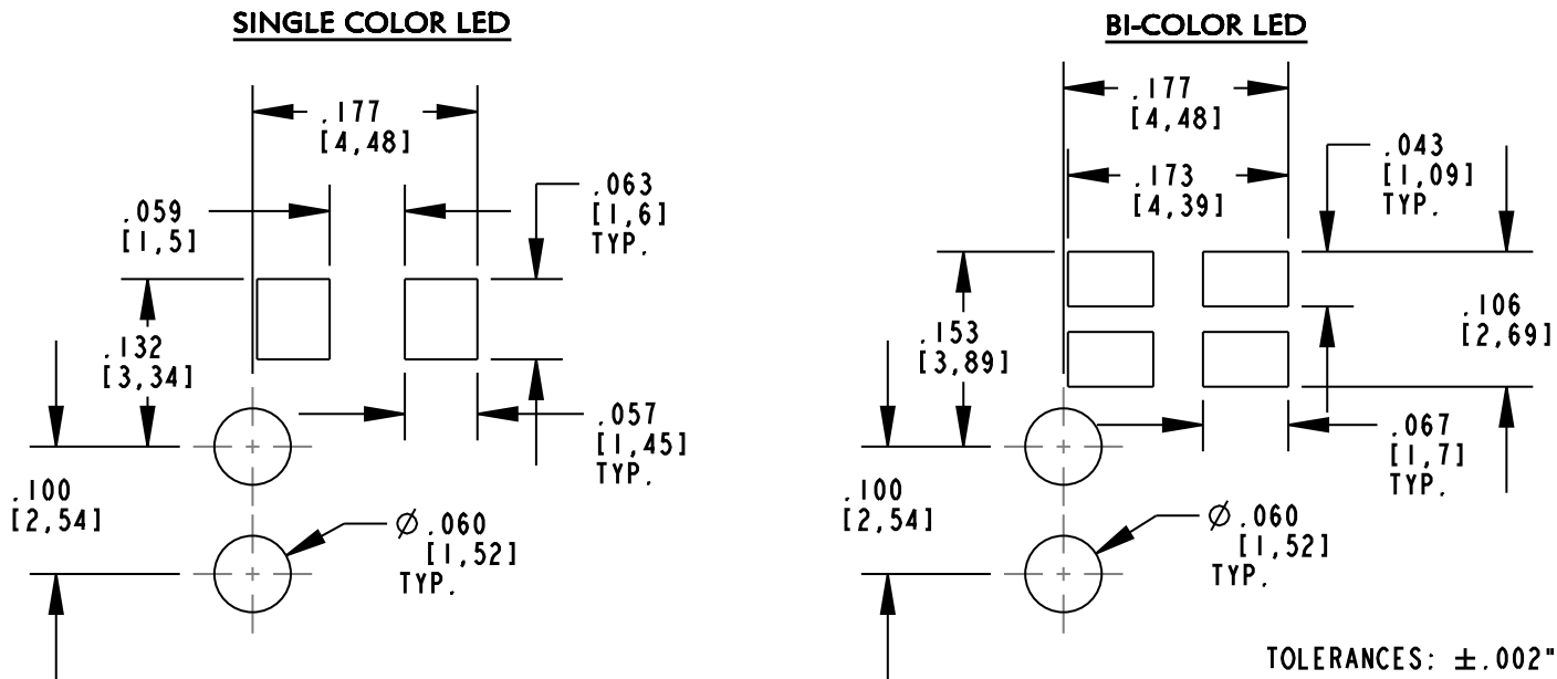
RECOMMENDED SOLDER PAD LAYOUT & HOLE PATTERN GAUGE
