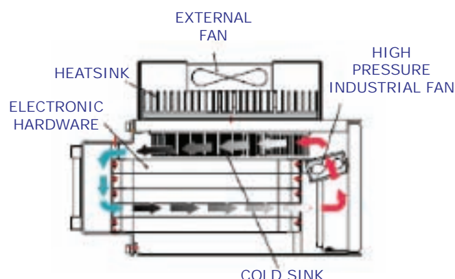
Cooling diagram showing airflow path for a typical indirect forced-air cooled ATR enclosure
