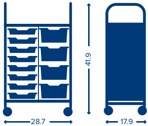
Callero Double Cart 8 Shallow & 4 Deep Trays
