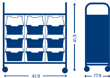
Callero Shield Tilted Tray Cart 9 Deep Antimicrobial Kiwi Jelly Tray
