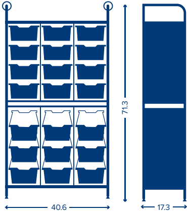
Callero Custom Tall Pick-Store Starter Unit 9 Tilting Deep & 12 Deep Trays
