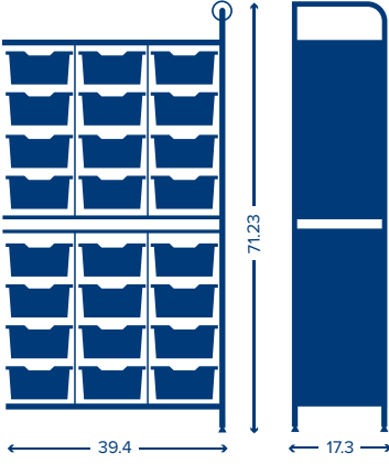
Callero Custom Tall High-Store Adder Unit 24 Deep Trays
