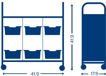
Callero Library Cart 6 Deep Trays
