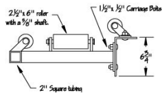
14" External Square Pipe Hoop Assembly Hardware Detail
