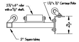
12" External Square Pipe Hoop Assembly Hardware Detail
