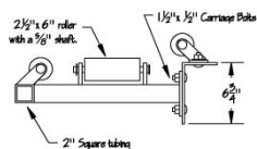
18" External Square Pipe Hoop Assembly Hardware Detail
