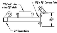
10" External Square Pipe Hoop Assembly Hardware Detail
