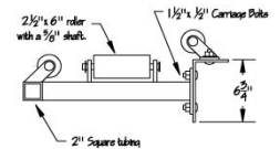
16" External Square Pipe Hoop Assembly Hardware Detail
