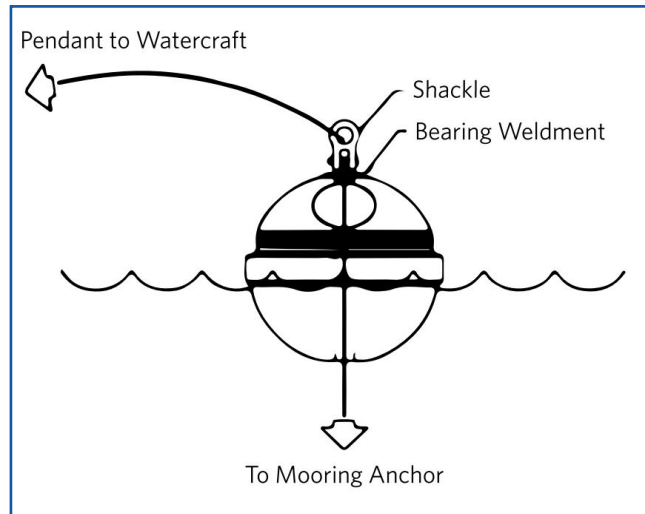
Diagram B: Pass-Through Mooring Hardware Installation
