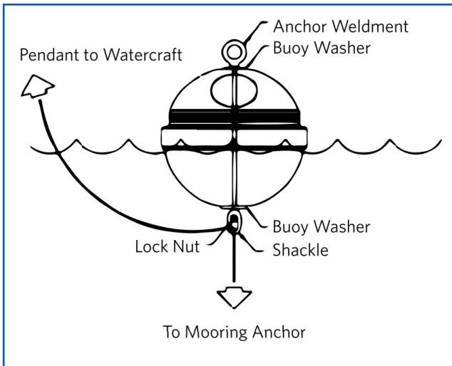
Diagram A: Fixed Mooring Hardware Installation
