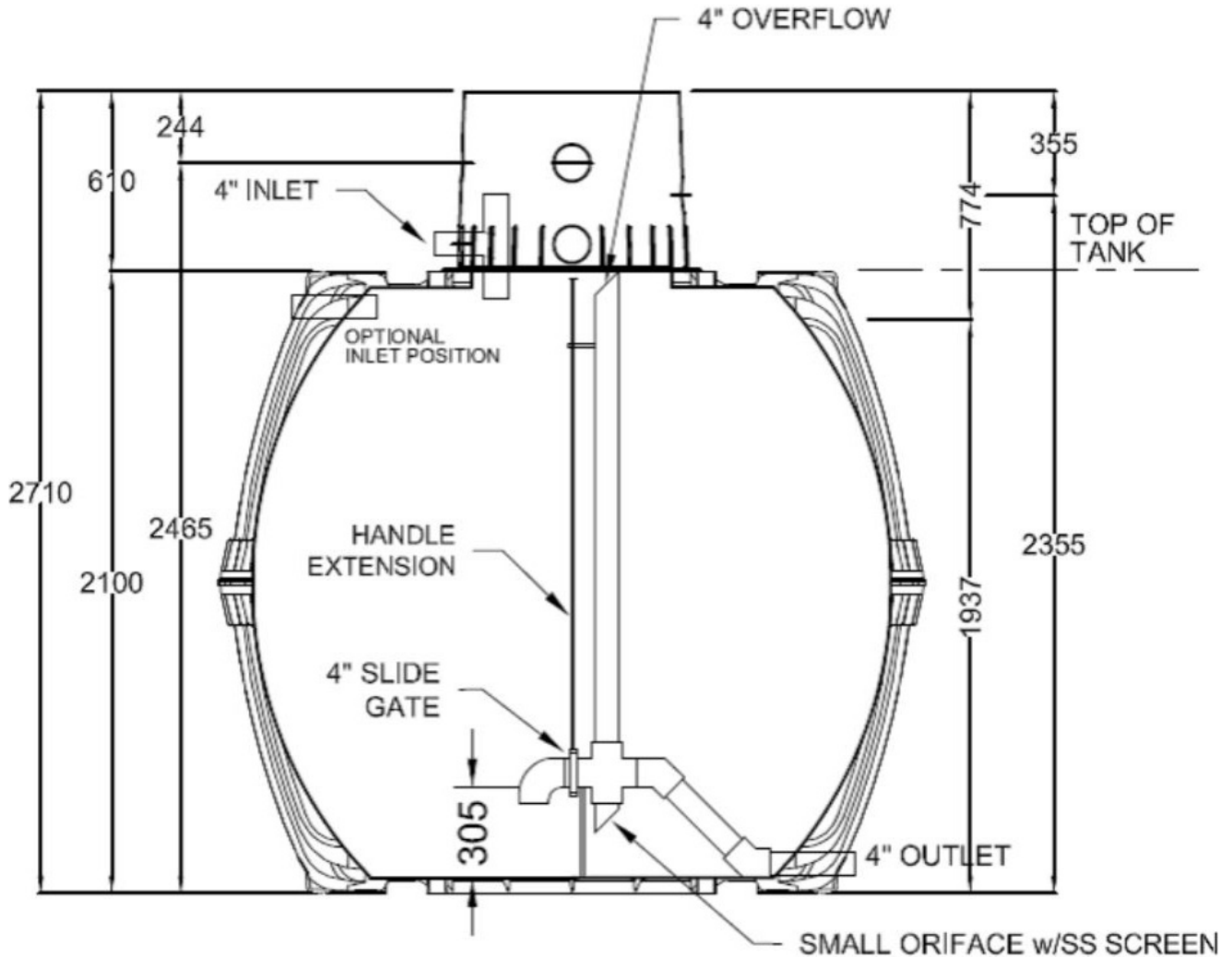
Common BARR StormStop Detention Tank Inlet / Outlet Module with Slow Release System.
