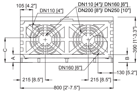
EcoBloc light system 402301 + 402300 + 402303
