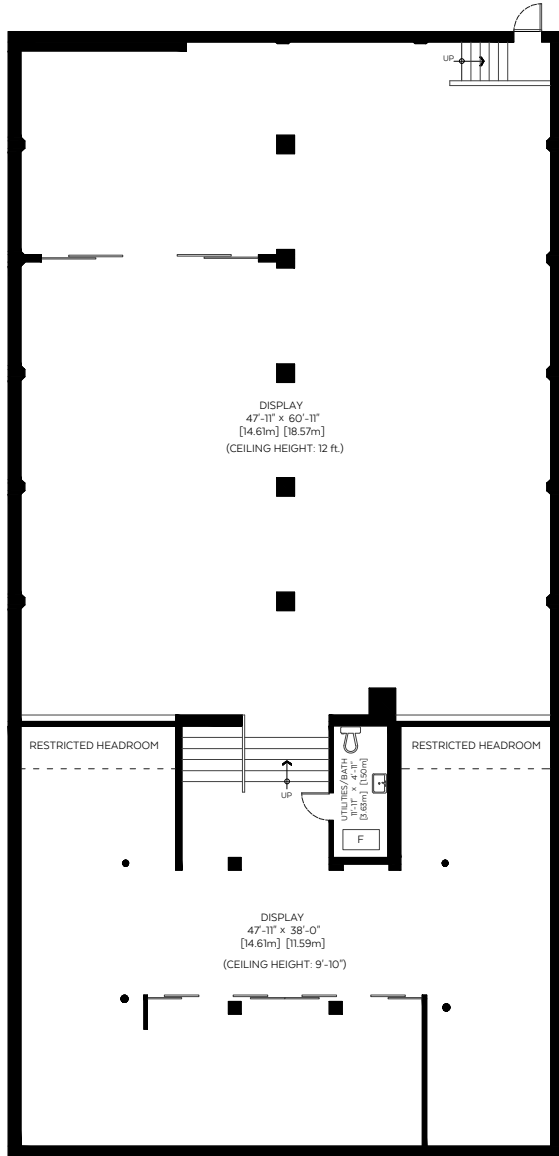
Lower Ground Floor Plan Floor Area: 4,981 sq.ft. Restricted Headroom Area: 127 sq.ft.
