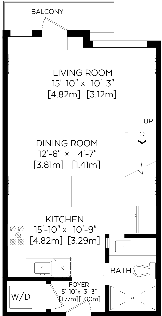
Main Floor Plan(Above Grd.) Floor Area: 454 sq.ft./42.18 sq.m.
