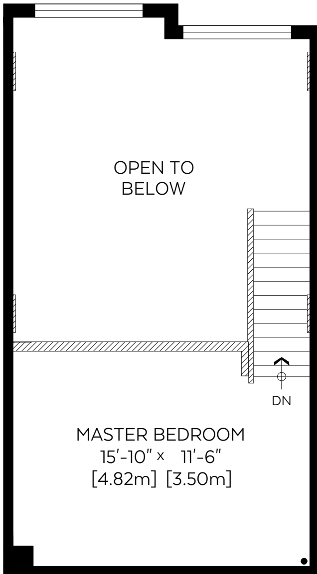
Upper Floor Plan(Above Grd.) Floor Area: 211 sq.ft./19.60 sq.m.
