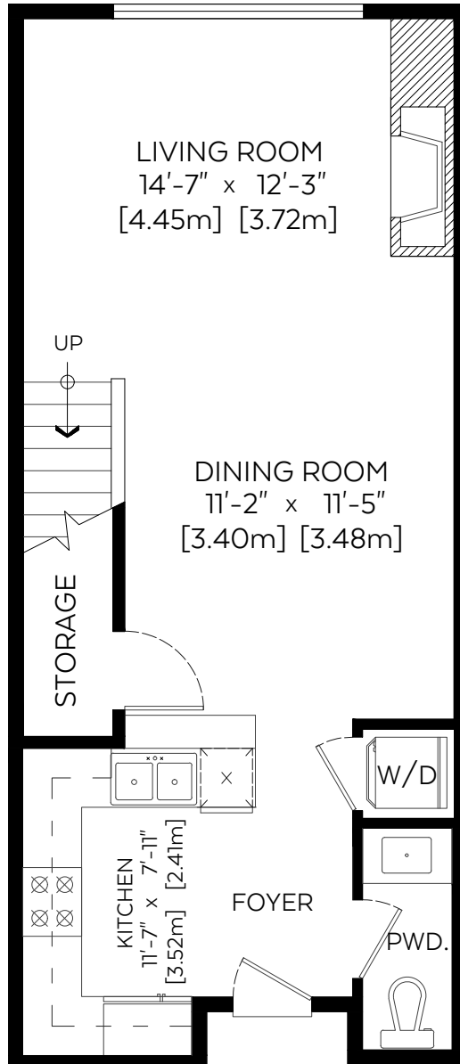
Main Floor Plan(Above Grd.)
