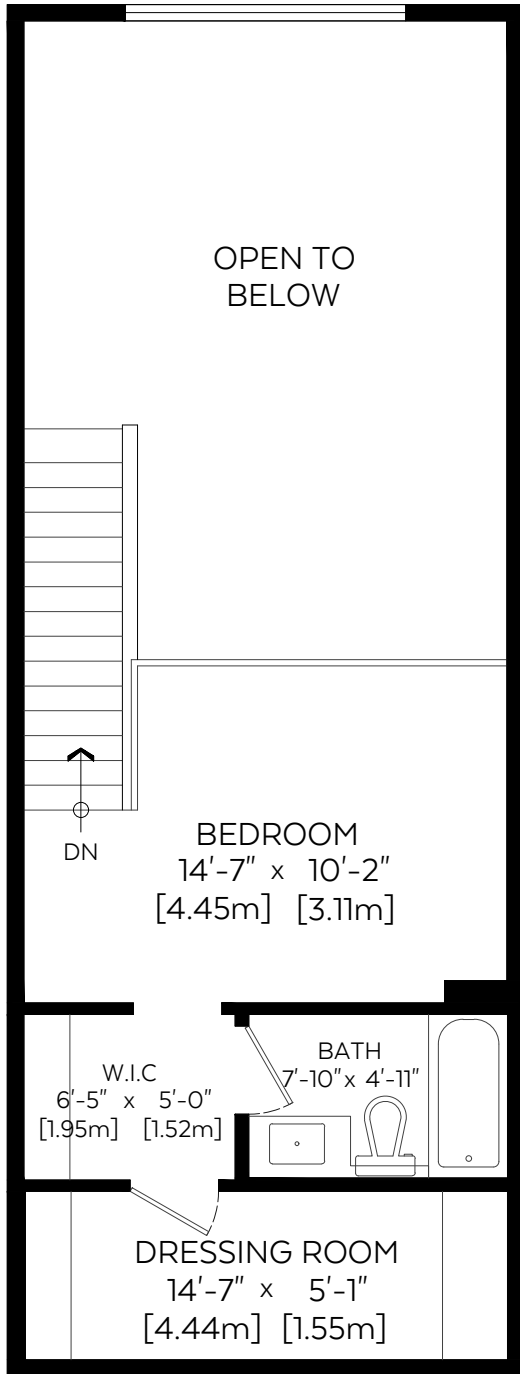
Upper Floor Plan(Above Grd.)
