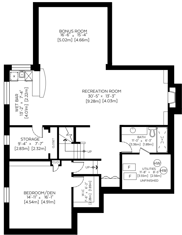
Lower Floor Plan (Below Grd.) Floor Area: 1,493 sq.ft./138.70 sq.m. Ceiling Height: 7'-6"
