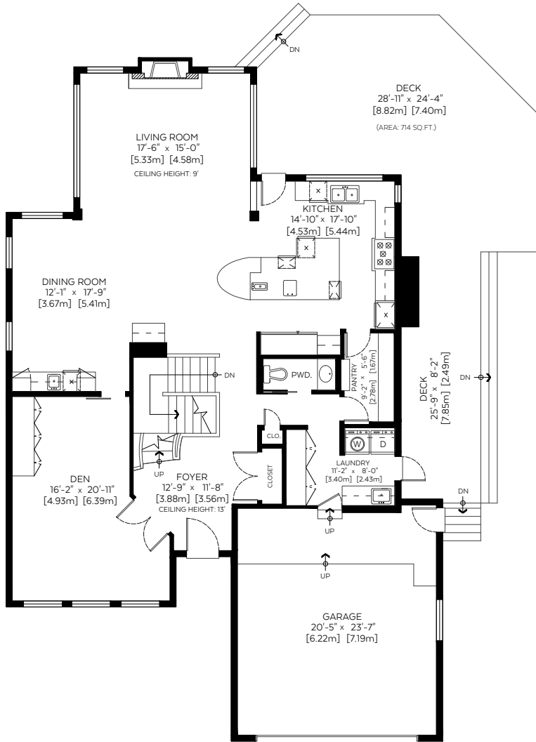
Main Floor Plan (Above Grd.) Floor Area: 1,774 sq.ft./164.81 sq.m. Ceiling Height: 8'
