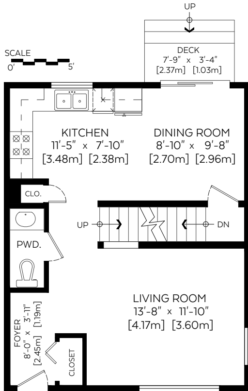
Main Floor Plan(Above Grd.)
