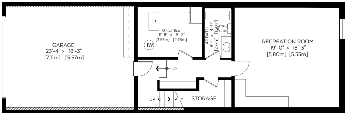
Lower Floor Plan(Below Grd.)
