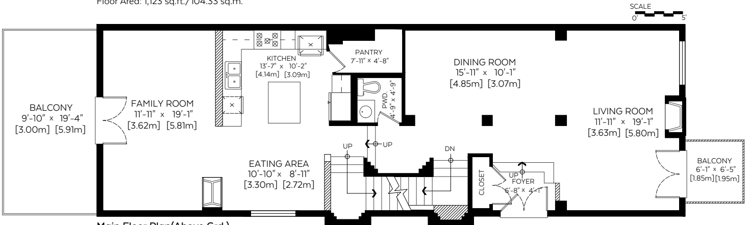
Main Floor Plan(Above Grd.)
