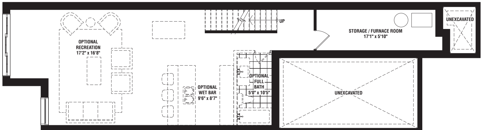
Basement - Option (1) 894 SQ. FT.
