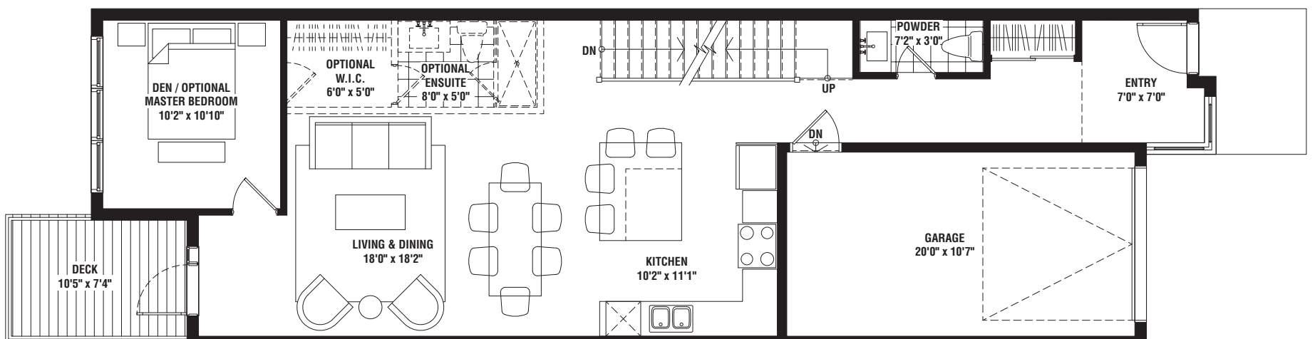
Ground Floor - Option (1) 942 SQ. FT.
