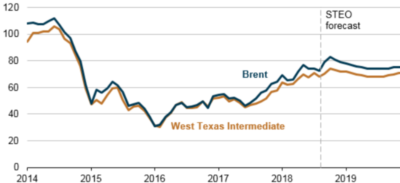
Monthly crude oil spot prices (Jan 2014-Dec 2019)
