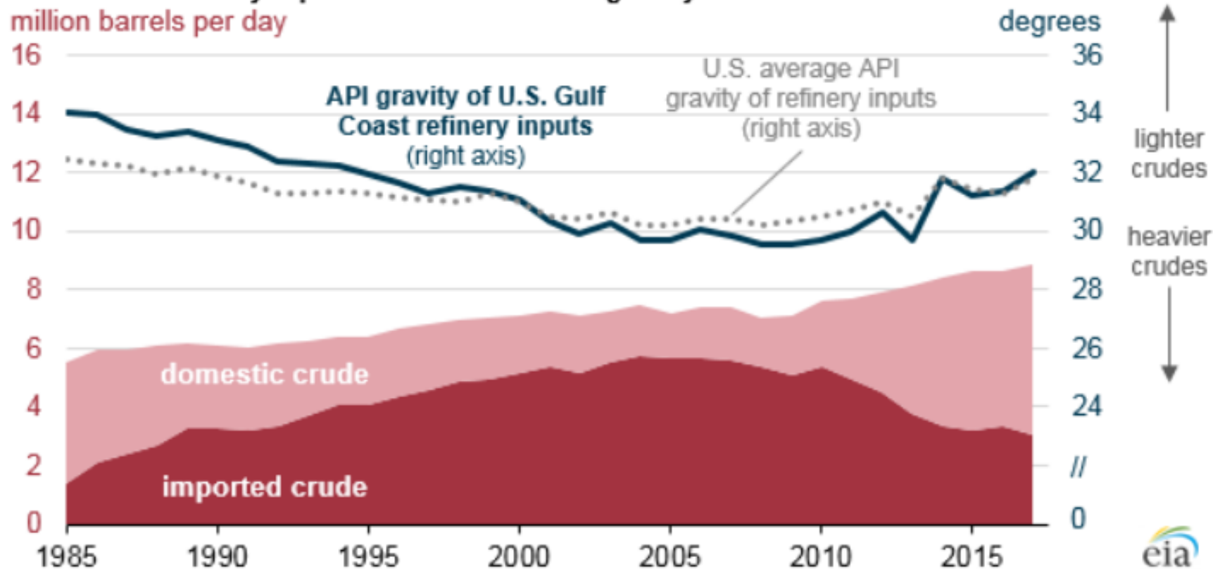
Gulf Coast refinery inputs and crude oil API gravity
