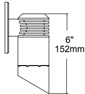
60° Angled Shroud
