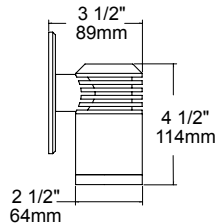
No Shroud
