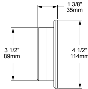
[S] Shallow (6 Cubic Inch)
