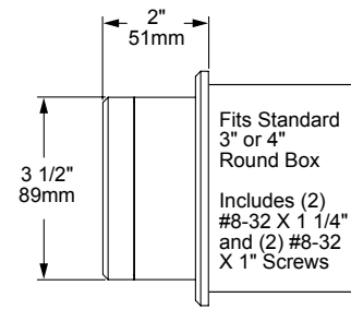
[D] Deep (10 Cubic Inch)
