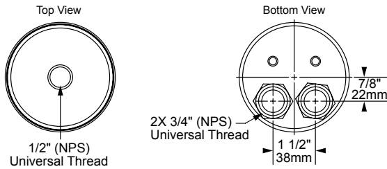
PM-1/2-1-BLP (Conduit not included)
