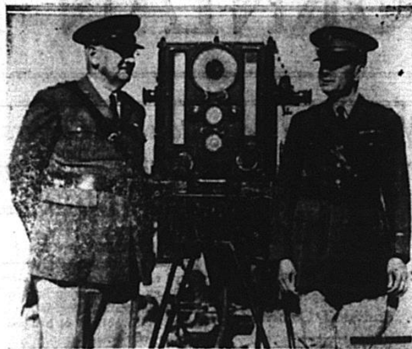
Pictured above is an instrument to detect and locate enemy aircraft and do everything else but fire anti-aircraft guns. Seen with the "mechanical brain" at Fort McArthur are, left, COL. CHARLES H. HILTON, post commander at Fort McArthur, and, right, LIEUT.-COL. HOMER R. OLDFIELD, commander of the Sixty-third Coast Artillery.
