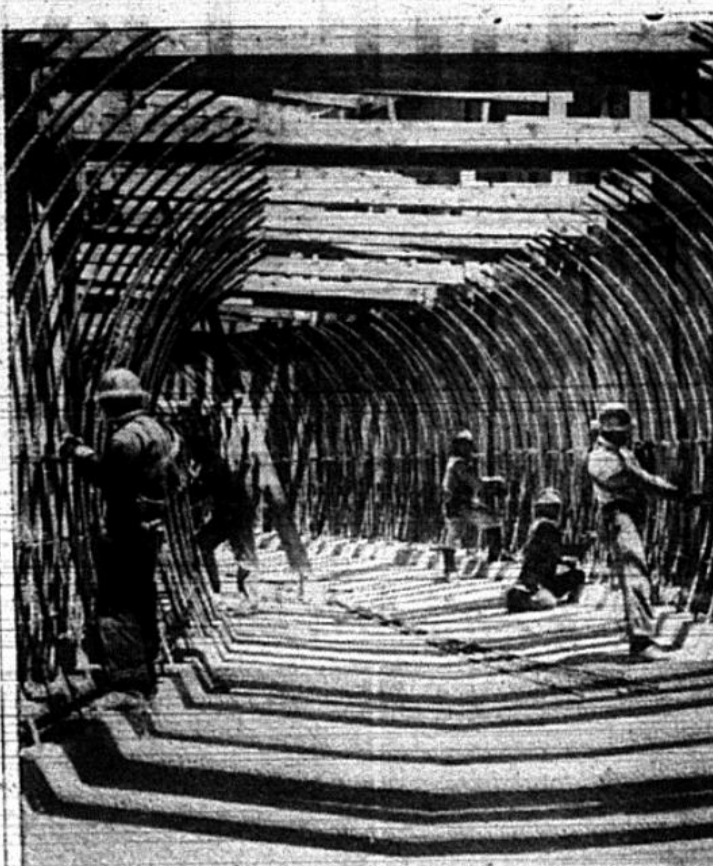
An Olympic boulevard storm drain is Los Angeles' weary answer to continual reputation-damaging floods. This vast underground structure is designed to drain saturated streets.
