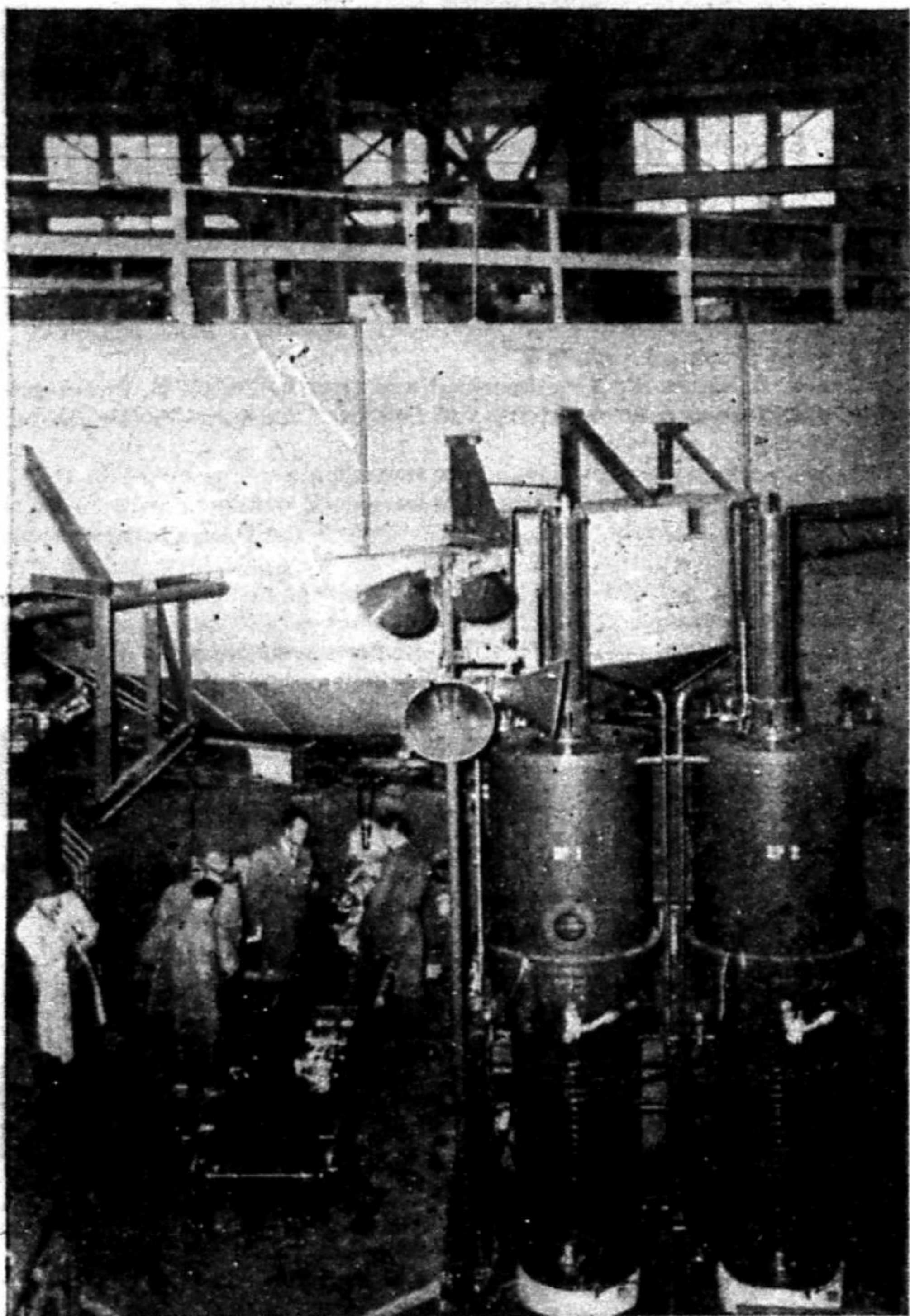
Two technicians are inserting an "ion" source into the newly completed 4,000 ton cyclotron. In the background is the upper part of the massive magnet with the railing running along the top and directly underneath is the accelerating chamber where the atomic "bullets" are whirled around to gain the necessary speed. Photo by Ken Silver '48
