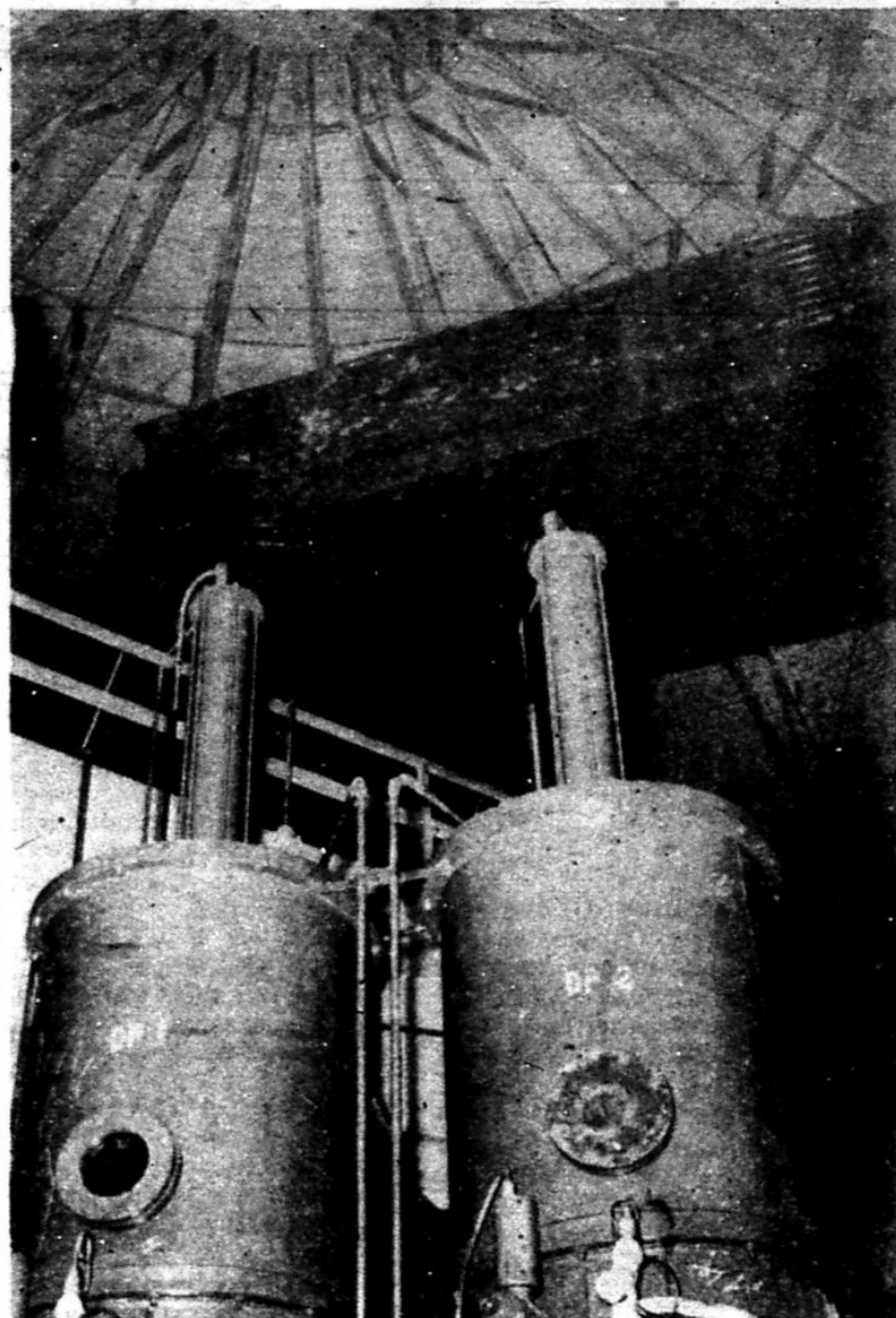
Above are shown two of the giant vacuum pumps that are necessary to produce the high vacuum needed inside accelerating chamber. They pump 300 cubic feet of air per second. Photo by Ken Silver '48
