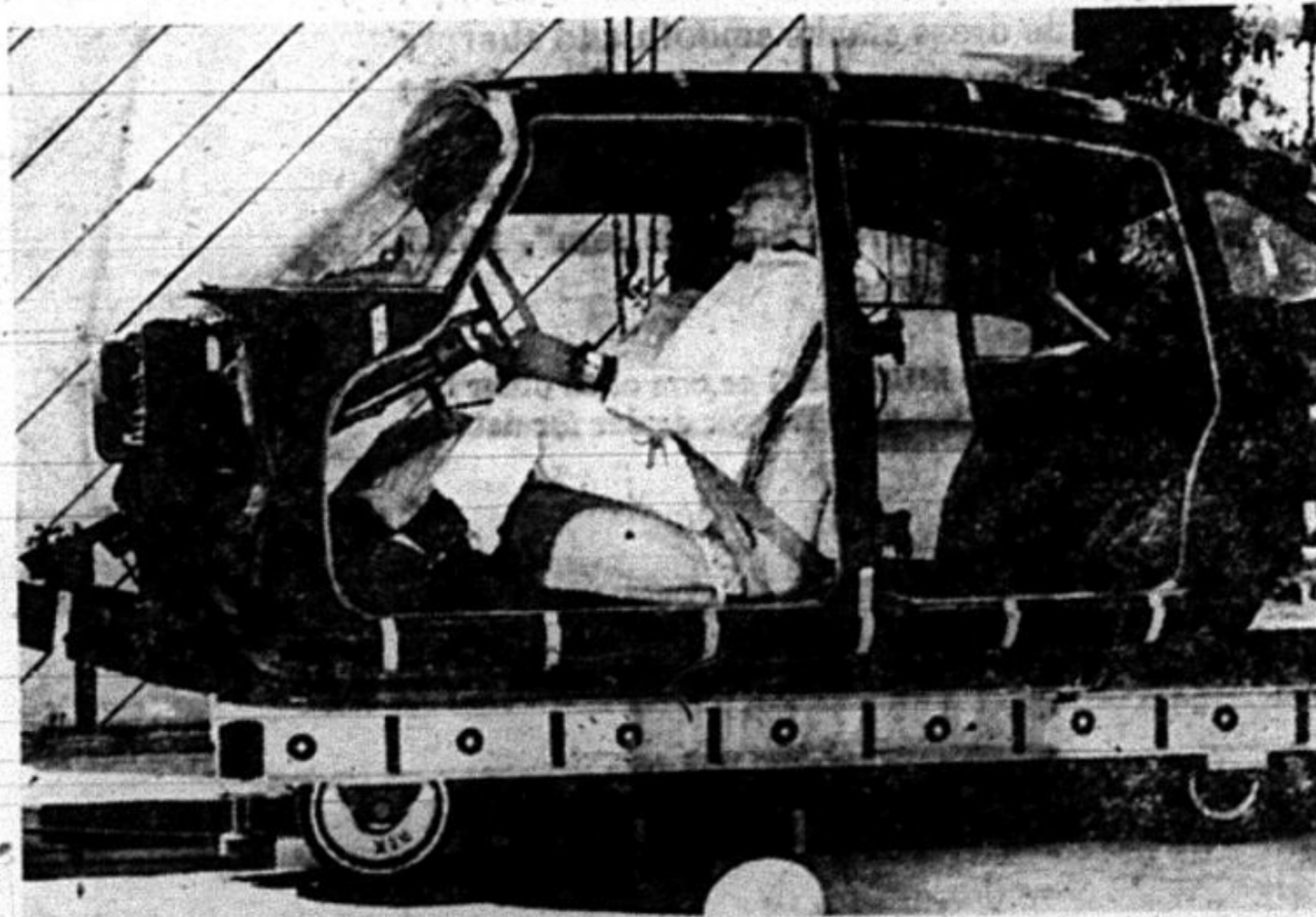
AUTO ACCIDENTS . . . The cab section of a car, mounted on a sled, can be brought to an almost instant stop, creating forces 50 times that of gravity, equal to those of the most severe collision.
