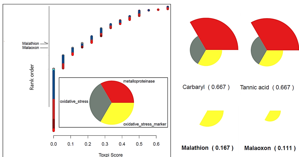
Fig. 4.6 ToxPi ranking for malathion, and its metabolite malaaxon, using ToxCast assay end-points mapped to oxidative stress
