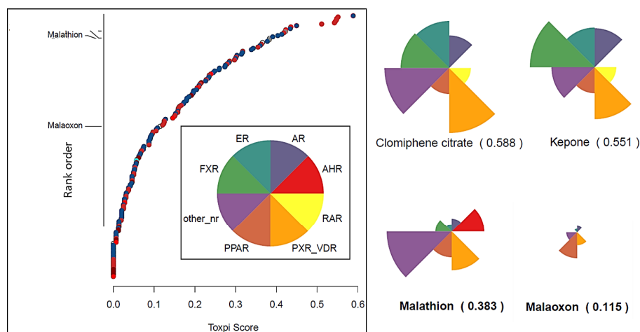
Fig. 4.8 ToxPi ranking for malathion, and its metabolite malaaxon, using ToxCast assay end-points mapped to modulation of receptor-mediated effects
