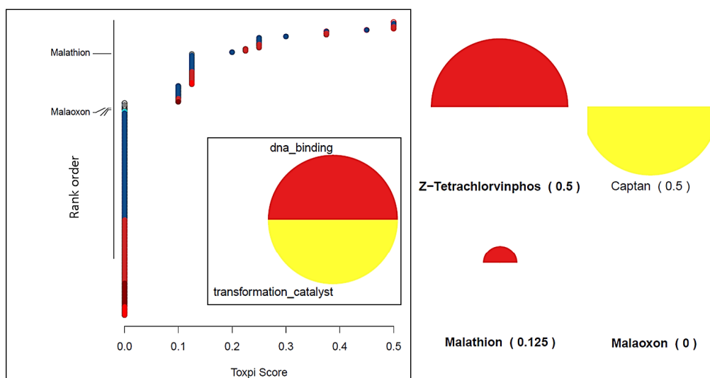
Fig. 4.5 ToxPi ranking for malathion, and its metabolite malaaxon, using ToxCast assay end-points mapped to epigenetic alterations
