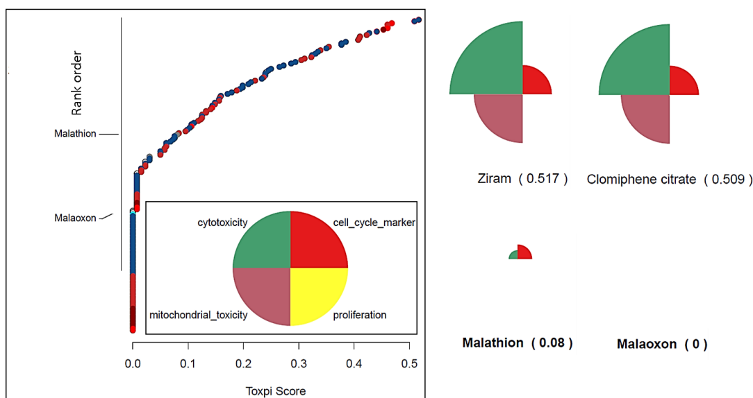
Fig. 4.9 ToxPi ranking for malathion, and its metabolite malaaxon, using ToxCast assay end-points mapped to cytotoxicity and cell proliferation
