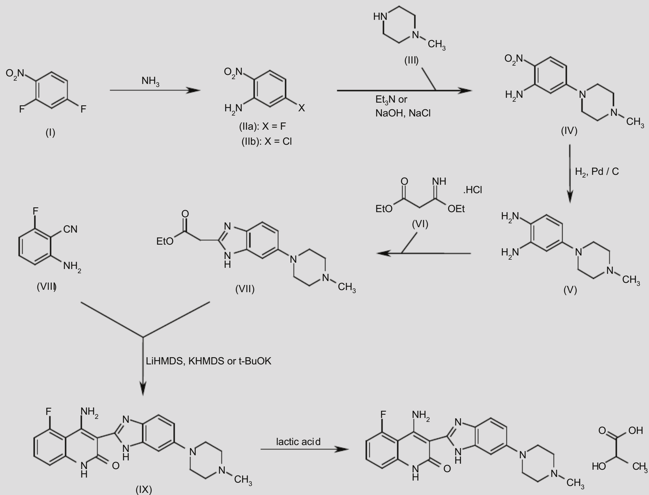
Scheme 1. Synthesis of Dovitinib Lactate
