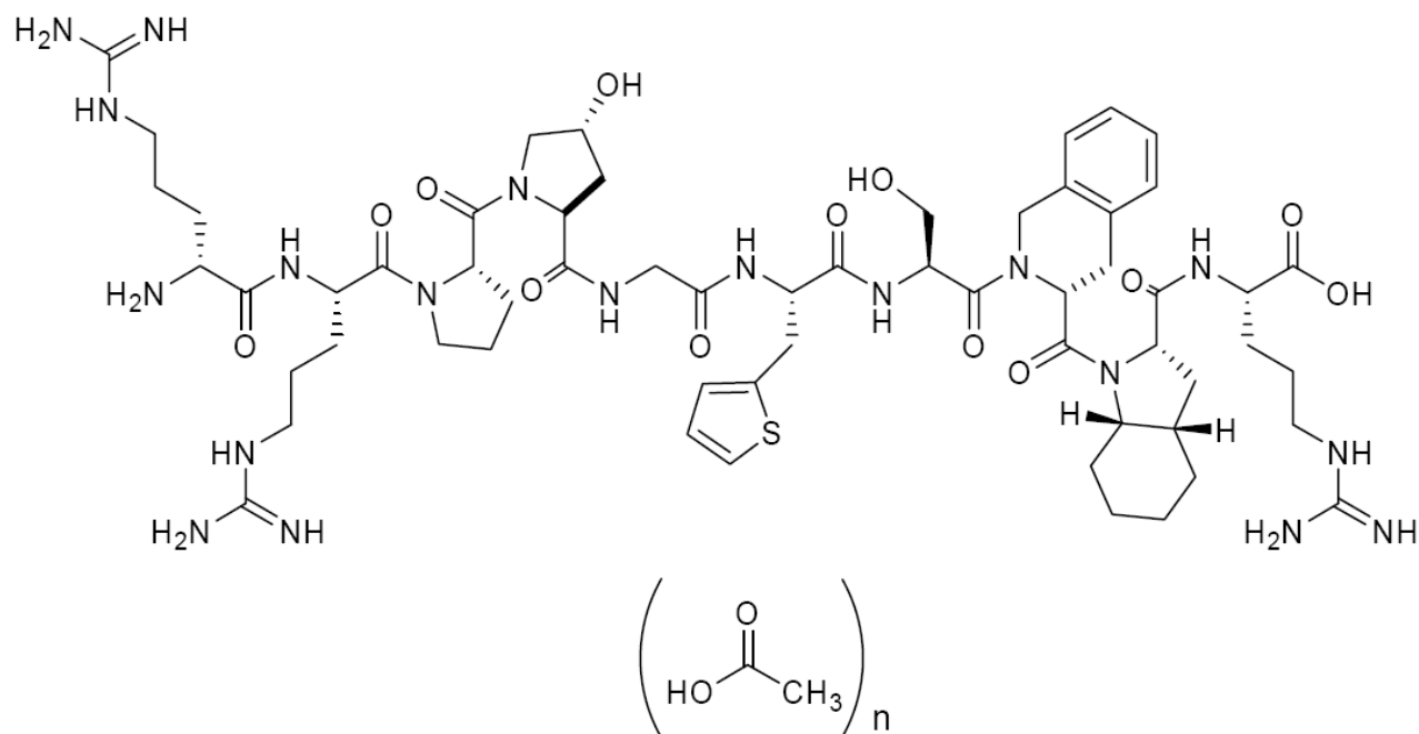
Figure 1 Chemical Structure
