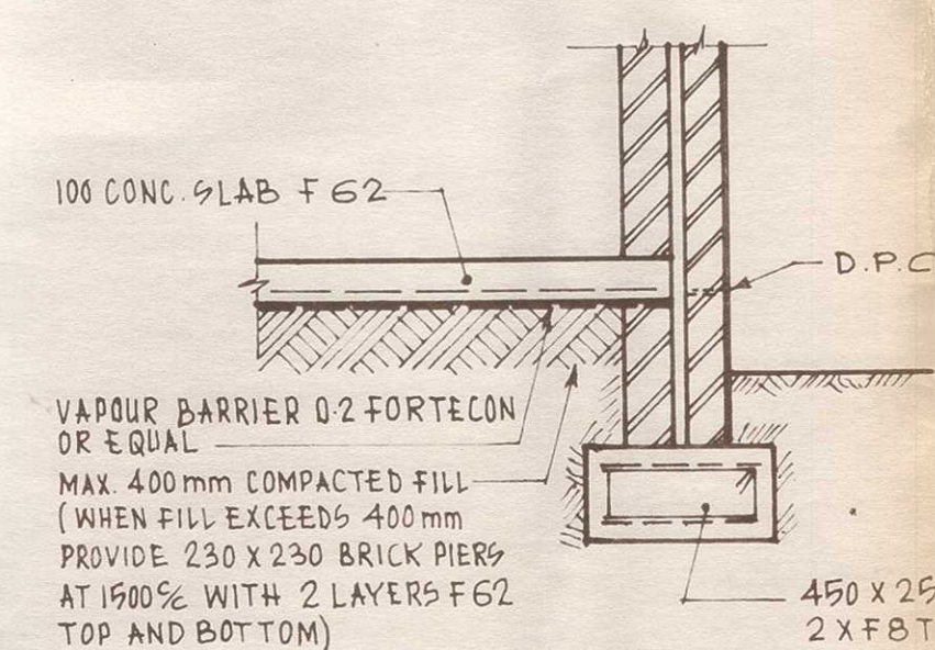
SLAB ON GROUND DETAIL
