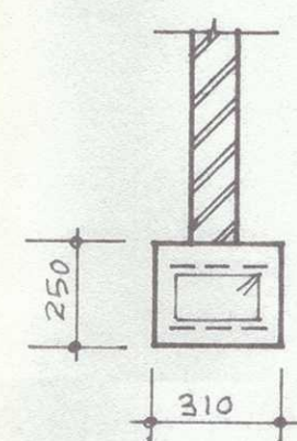
TYPICAL FOOTING DETAIL
