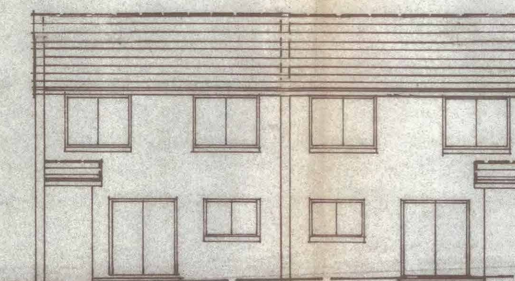
CONT. REAR ELEVATION BLOCK 2 (UNITS 7,8,9,10)
