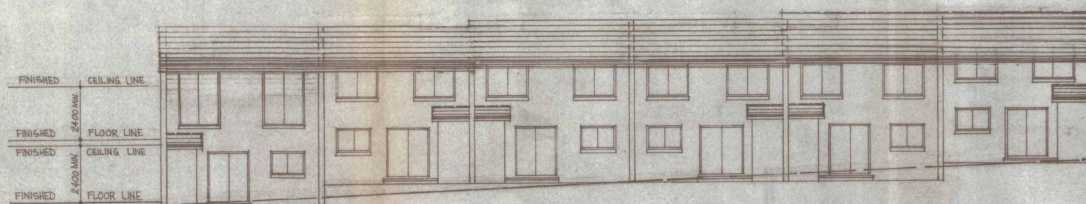
REAR ELEVATION BLOCK 3 (UNITS 11,12,13,14,15,16)
