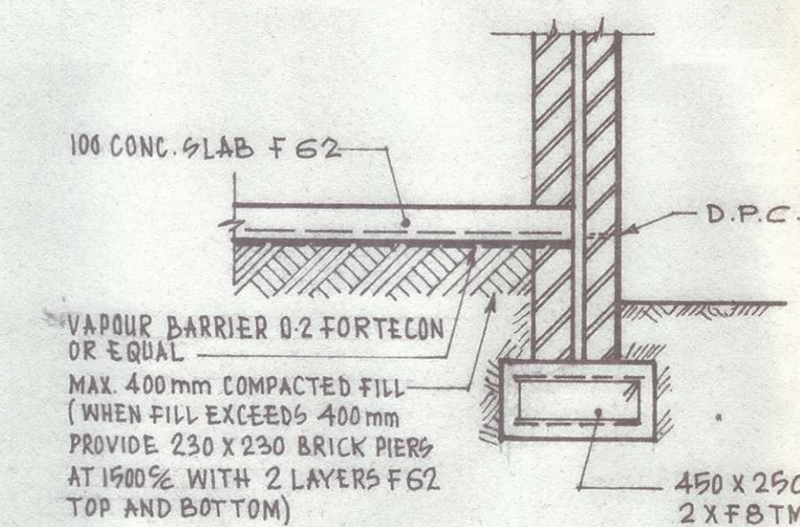
SLAB ON GROUND DETAIL
