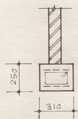
TYPICAL FOOTING DETAIL
