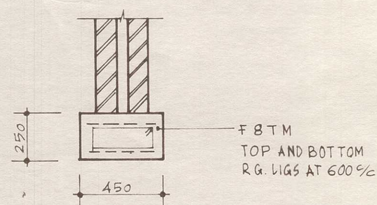
TYPICAL FOOTING DETAIL
