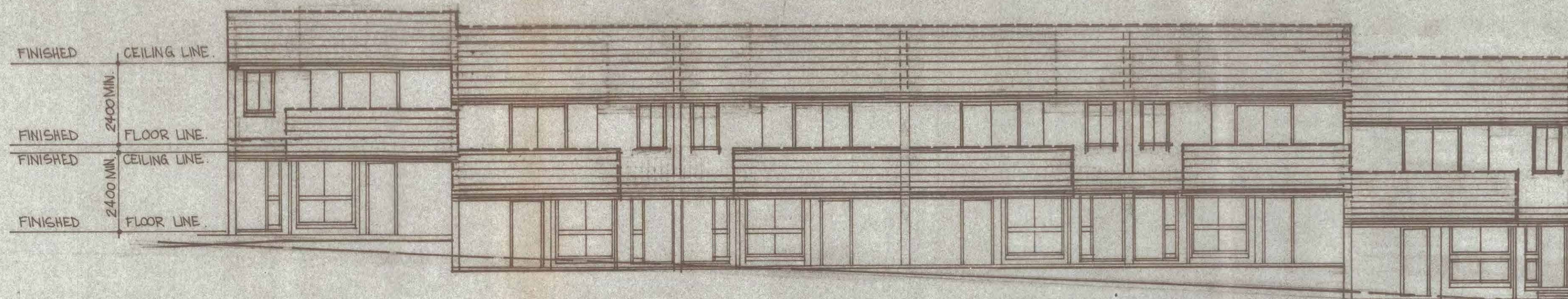
FRONT ELEVATION BLOCK 1 (UNITS 1,2,3,4,5,6)
