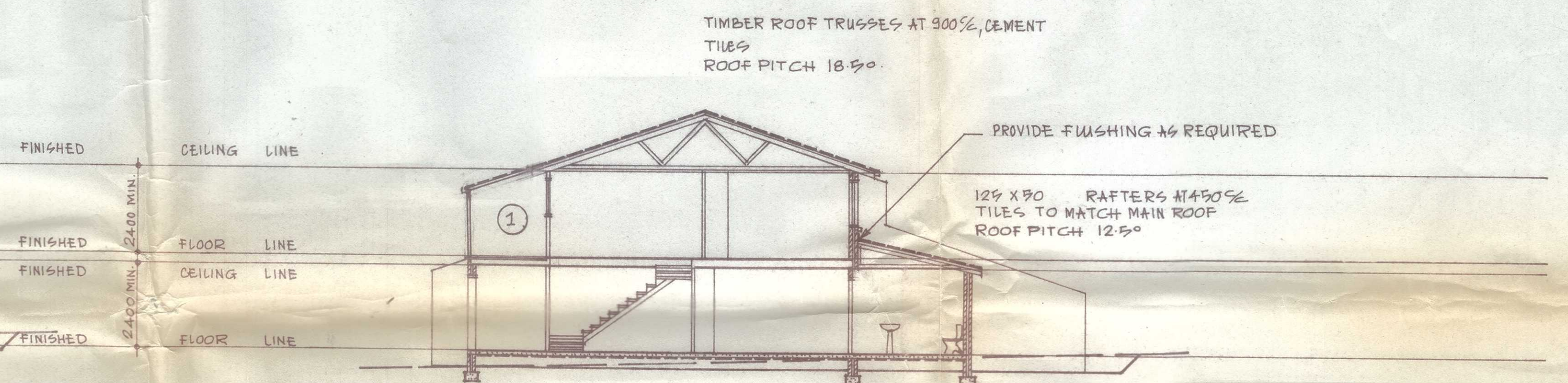
SECTION B B
