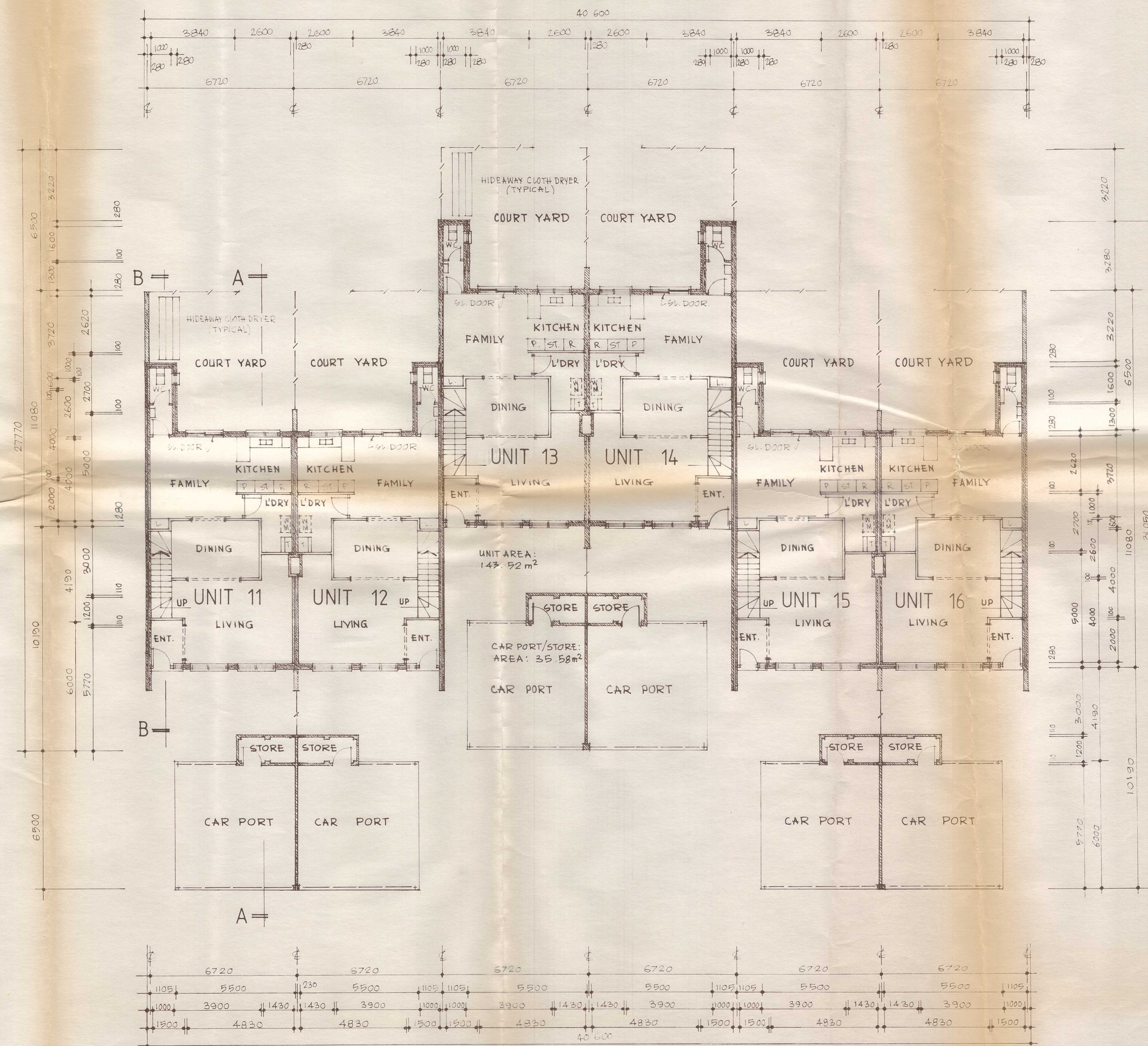
GROUND FLOOR PLAN BLOCK 3 UNITS 11, 12, 13, 14, 15, 16
