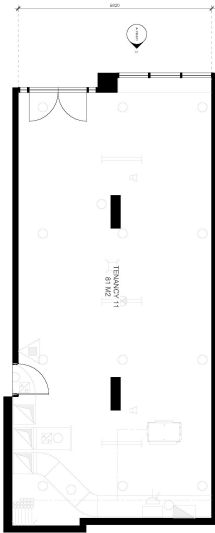
1 SHOP 11 GROUND FLOOR PLAN 1:100
