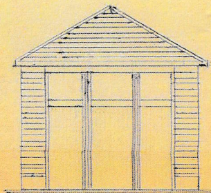
FRONT ELEV
