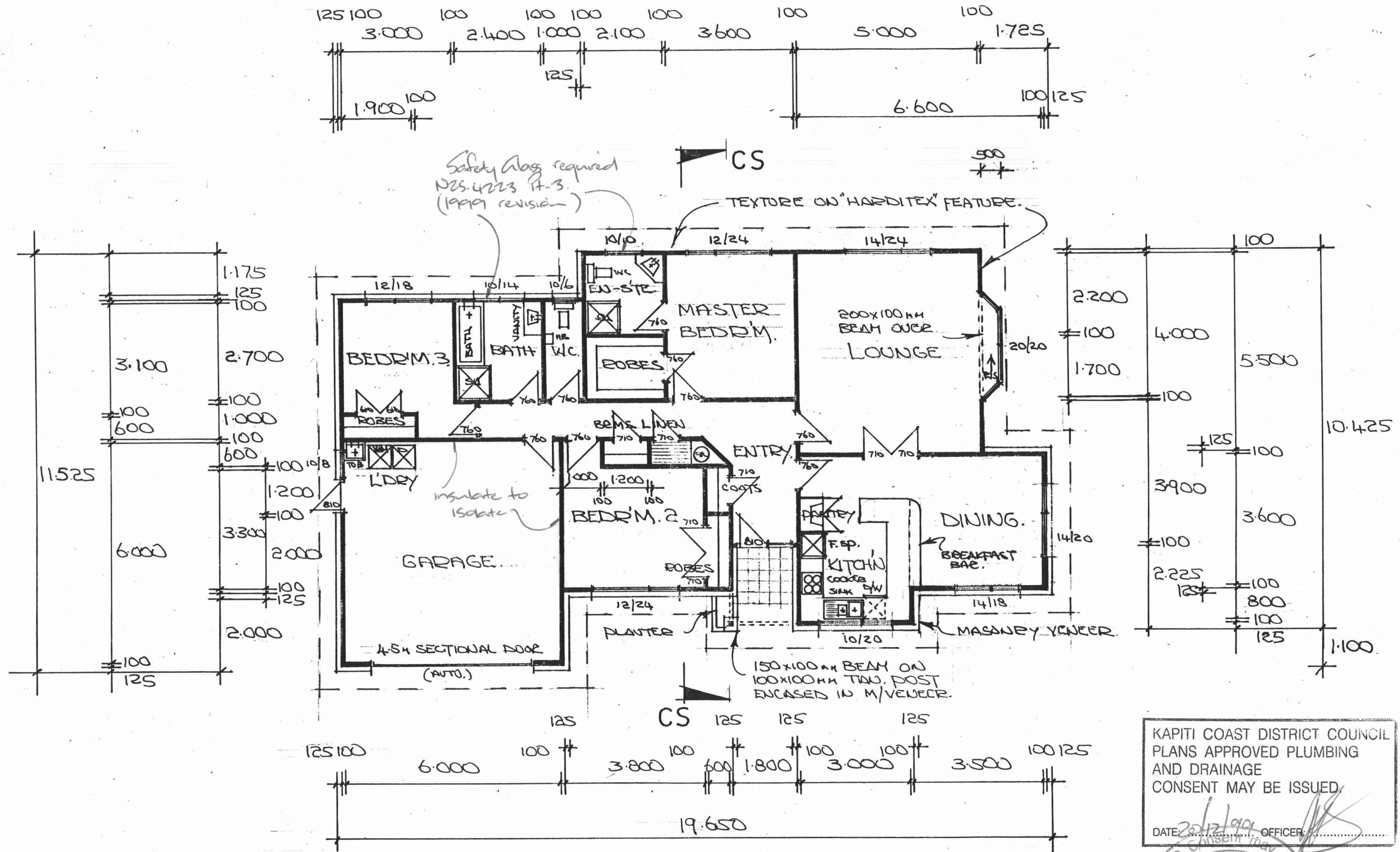
FLOOR PLAN. 1:100.
