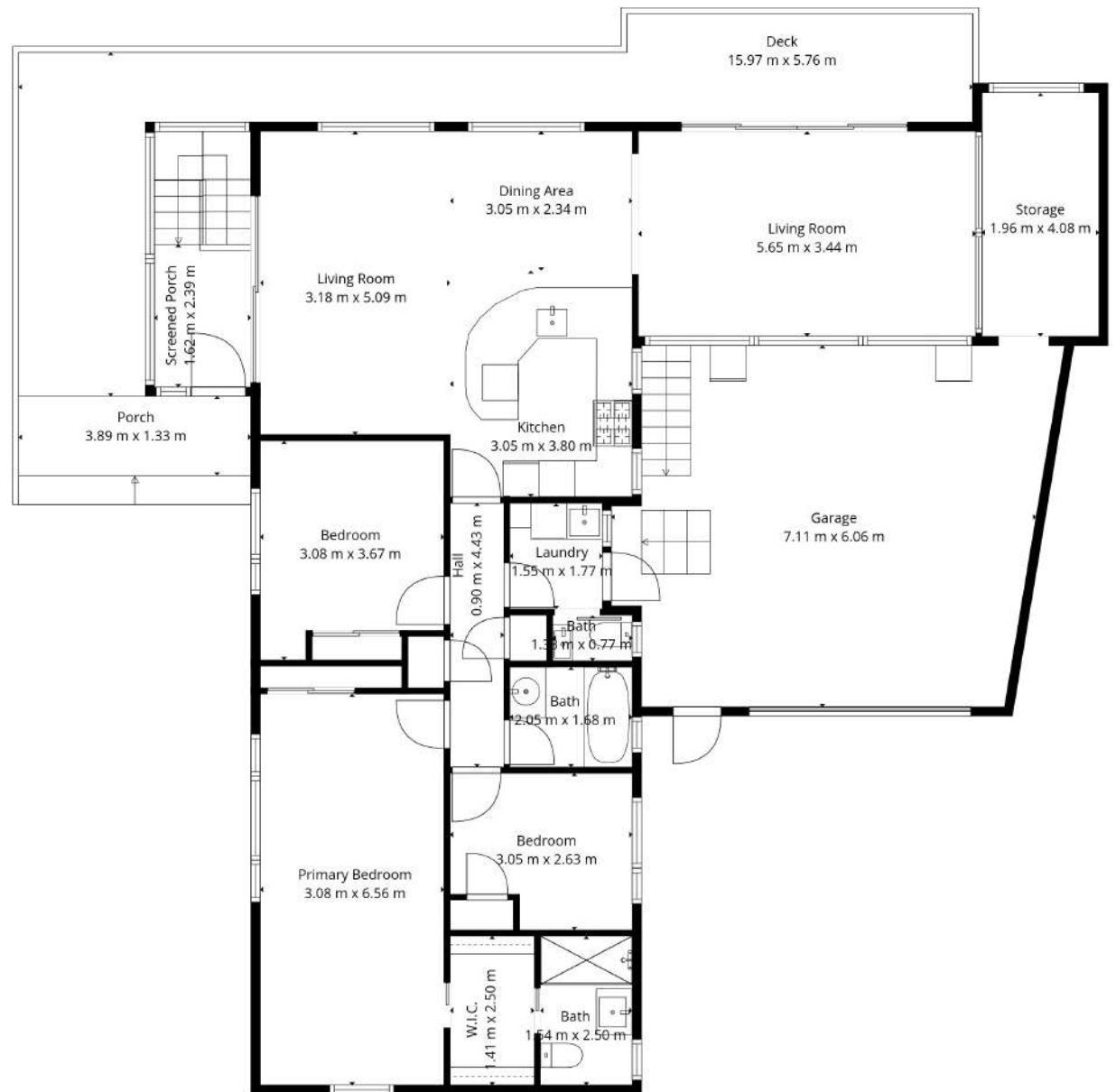
2nd Floor
