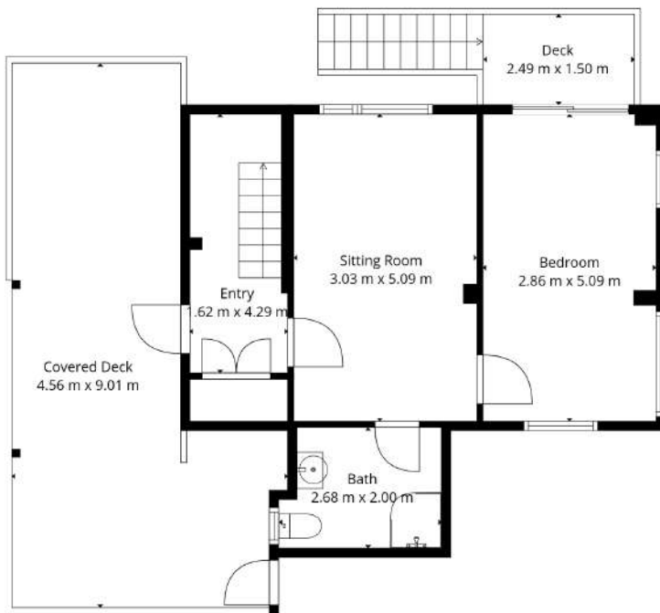
1st Floor
