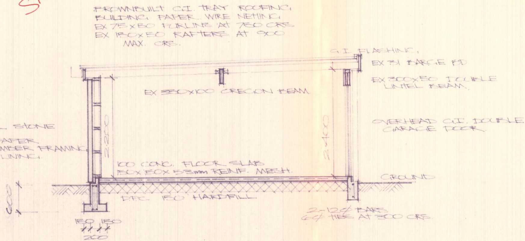
TYPICAL GARAGE CROSS SECTION
