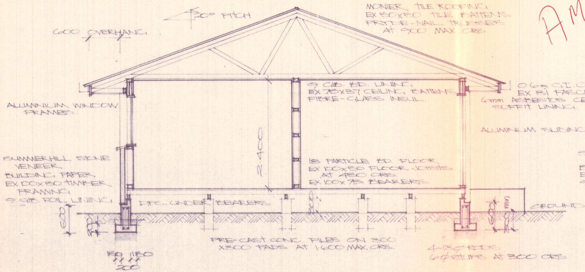
TYPICAL FLAT CROSS SECTION
