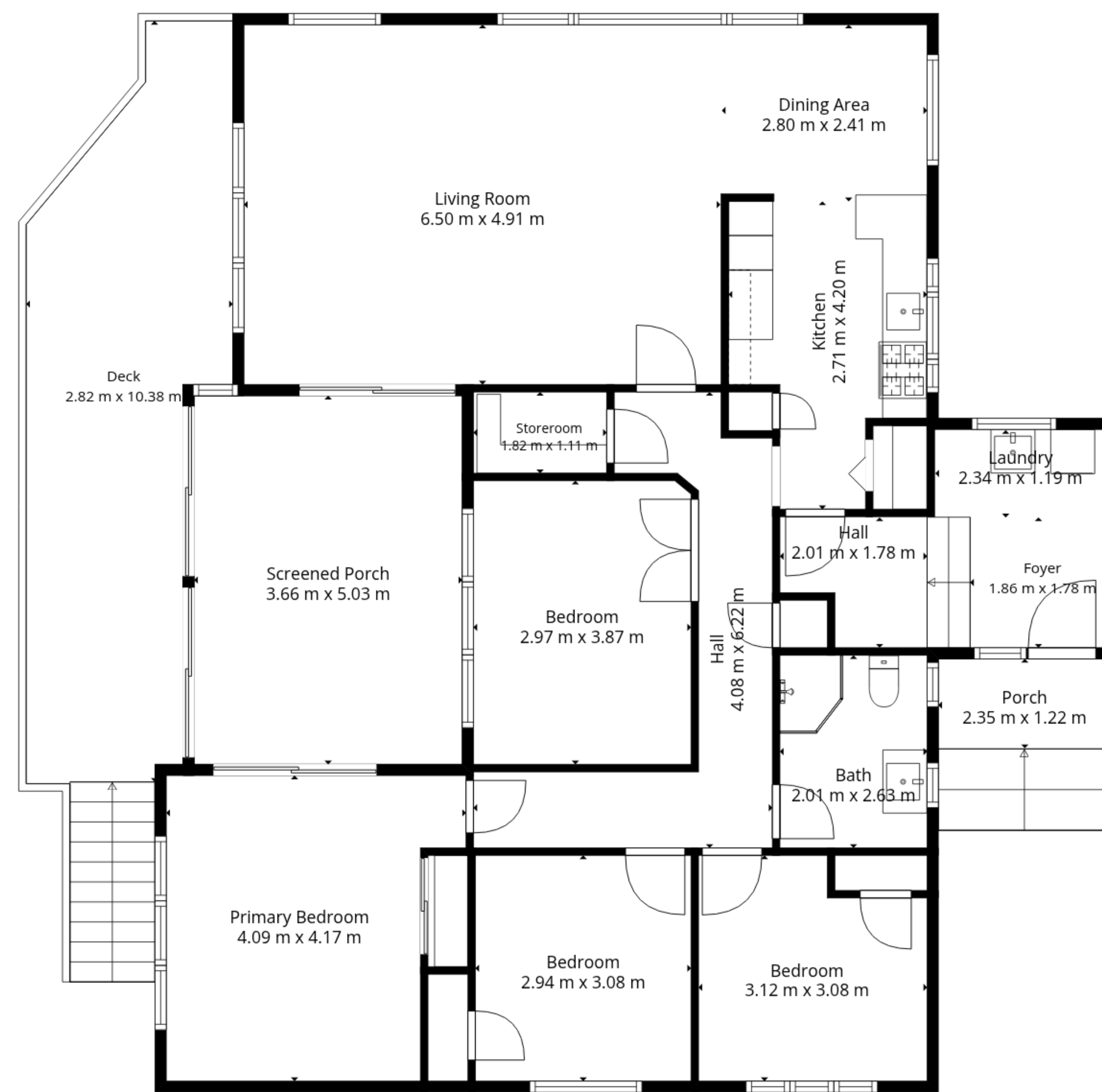
2nd Floor
