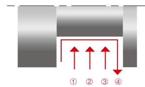
Grooving(Roughing) &Turning(Finishing)
