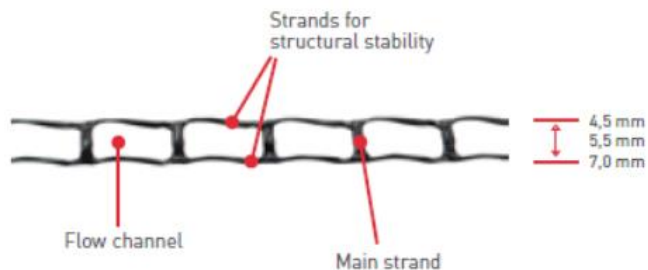
Figure 9 Cross section of the geonet and range of thicknesses
