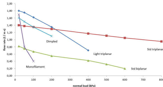
Figure 11 Comparison of short-term flow capacity for various drainage composites, gradient i=1 and Hard-Soft boundary conditions, in accordance with ISO 12958
