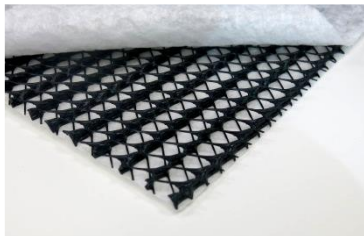
Figure 8 New tri-planar geonet
