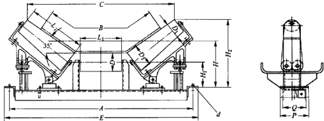
十三、锥形上调心托辊 Self Aligning Taper Idler Set
