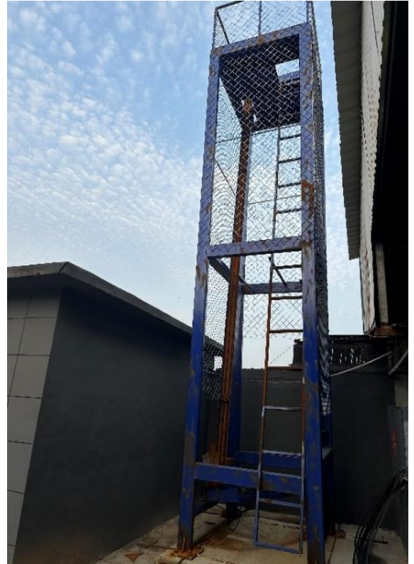
Dropping Tester
