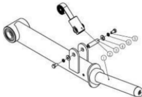
Weight Frame second Assy
