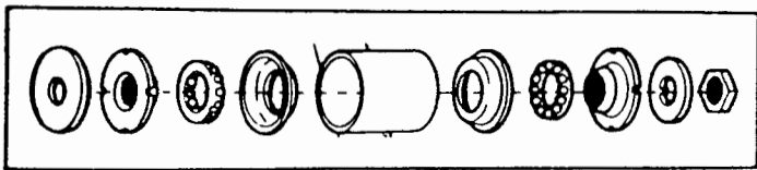
CRANK ASSEMBLY (47)
